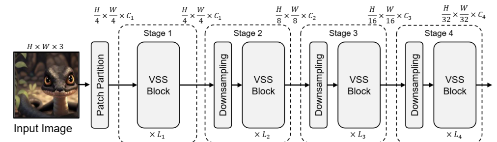
(a) Architecture of VMamba
