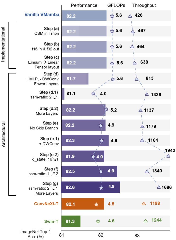
(e) Performance Comparison
